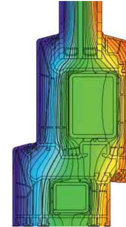
Isothermal flow Schüco LivIng AS front door
